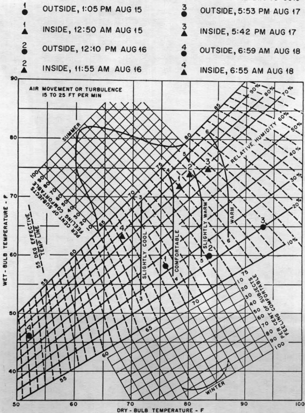
Fig. 4.19. Eight approximately paired temperatures ( ^{\circ} F), four outside and four inside the Log-Covered Trench Shelter with seven occupants.
